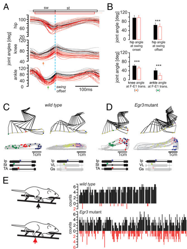
Fig. 2. Kinematic and functional consequences of the absence of early TA offset. (A) Average angular movement of three leg joints during walking of wild types (black lines, n = 16 animals) and Egr3 mutant mice (red lines, n = 18 animal). Bold lines are pooled averages from all mice and thin lines are averages from individual animals. Horizontal red bars on Top indicate the average duration ( \pm SD) of swing (sw) and stance (st) phases, together with the similar data from wild types (black bars). (B) Comparison of mean ( \pm SD) of maximal and minimal hip joint angles ( Top graphs) and minimal joint angles of knee and ankle joints during swing phase ( Bottom graphs). ***P < 0.001 . (C and D) Stick reconstruction of swing phases on Top and toe trajectories of multiple steps overlapped with EMG events from two steps from a wild-type (C) and an Egr3 mutant (D) mouse. Sketches on the Bottom indicate the color-coded EMG events in Upper diagrams. Black and gray bars indicate flexor and extensor activity, respectively. The large rectangle in the background is the average step cycle, shaded area indicating the swing phase. (E) The Egr3 mutant mice make more errors during walking on a horizontal ladder, determined as more frequent foot droppings between rungs than in wild types. Each bar indicates number of steps that landed safely on a rung (black bars) or dropped between the rungs (red bars) counted during one run ( N = 13 for wild type, 15 for mutant).
